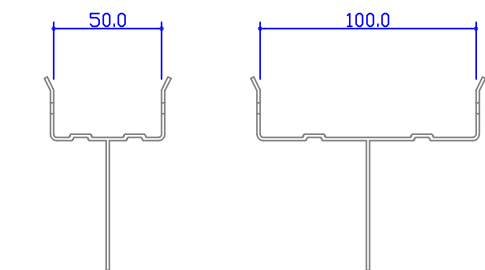
CARRIER AVAILABLE IN 75mm-150mm LENGTHS TO SUIT DOUBLE AND SINGLE BRACKET SIZES
